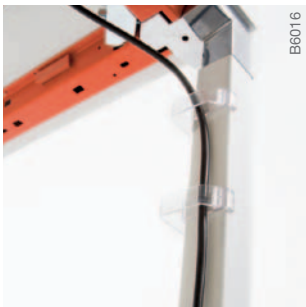
Cable clips, translucent plastic, attached to leg.
